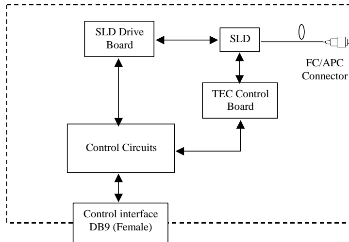
Figure 1 Configuration of IPSDS1602-xxxxx SLD light source module
